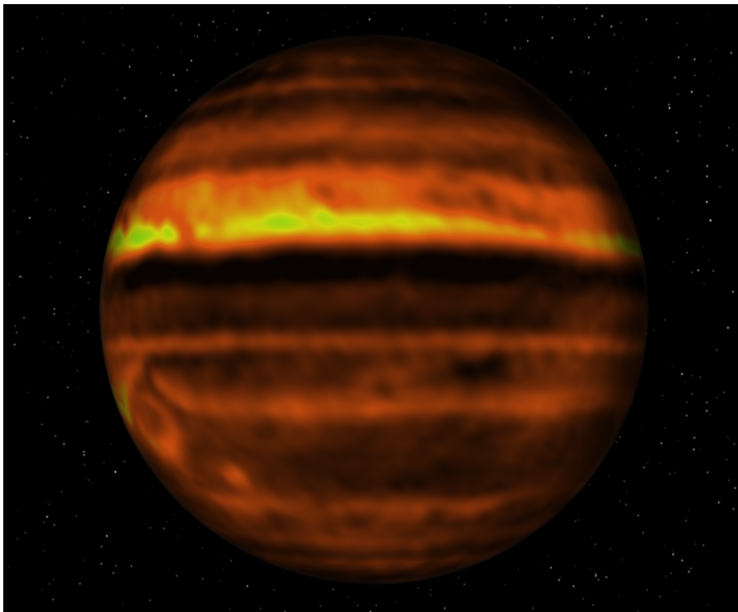
Figure 25: Spherical image of Jupiter showing the distribution of ammonia gas below Jupiter's cloud deck. (Credit: ALMA (ESO/NAOJ/NRAO), I. de Pater et al.; NRAO/AUI)
