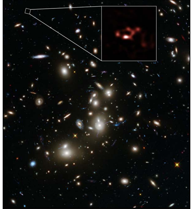
Figure 14: The inset of this HST image galaxy cluster Abell 2744 shows an ALMA image of the z=8.38 gravitationally-lensed galaxy A2744_YD4. At this distance, the universe was a mere 600 million years old, and yet the ALMA observations show that the galaxy is rich in dust. (Credit: ALMA (ESO/NAOJ/NRAO); NASA; ESA; ESO; D. Coe (STScI)/J. Merten (Heidelberg/Bologna); Laporte et al., 2017, ApJ , 837, L21)
