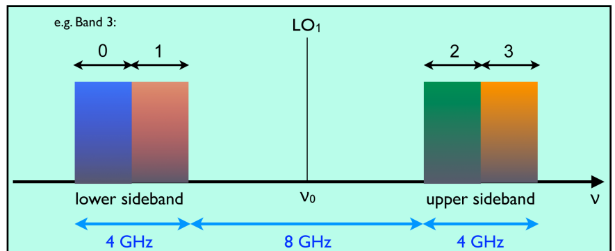
Figure 31: A graphical view of basebands and sidebands. Basebands may be tuned to overlap if the user wishes, or may be located so as to maximize the total bandwidth (as shown). Each baseband may be further subdivided into as many as 8 spectral windows. Up to four spectral windows per baseband will be available during Cycle 8.
