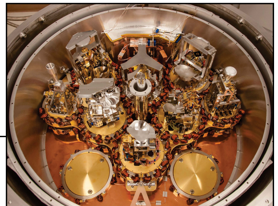
Figure 33: An open cryostat fitted with receivers covering Bands 3 through 10. The two “empty” slots will eventually be occupied by Bands 1 and 2 receivers, giving ALMA complete spectral coverage from \sim 30 GHz to nearly 1 THz. (Credit: ALMA (ESO/NAOJ/NRAO))
