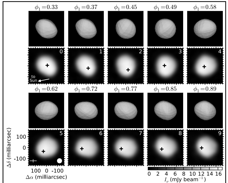
Figure 24: Asteroid 3 Juno was observed in October 2014 during the commissioning period of the ALMA long baseline campaign. Over the course of the observations, the achieved resolution varied from 32 \times 24 mas to 42 \times 36 mas, differing mostly due to changes in phase stability as the observations spanned the transition from night through dawn and into daytime. The baselines used to achieve this resolution ranged from 26 m to 13 km. The observations spanned 10 epochs, covering 60% of the 7.2h rotation period. (Credit: ALMA Partnership et al., 2015, ApJ, 808, L2)
