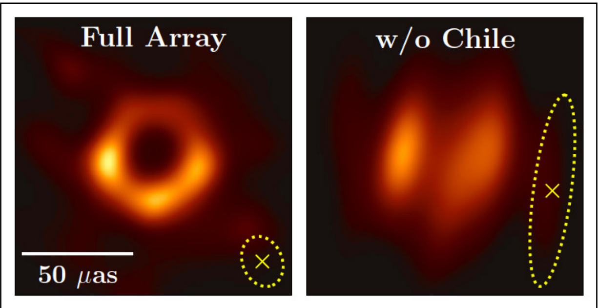
Figure 10: This image (left) of the event horizon from the supermassive black hole at the center of the M87 galaxy was created by a consortium of observatories across the globe, and won the Event Horizon Telescope (EHT) team the $3M 2020 Breakthrough Prize in Fundamental Physics. ALMA played a critical role in the EHT, providing both greatly enhanced sensitivity and critical baselines; the right panel shows how the image would have appeared without the Chilean observatories (ALMA + APEX). Astronomers can apply to use the EHT for 1 mm Very Long Baseline Interferometry using the Cycle 8 OT. (Credits: EHT Collaboration)
