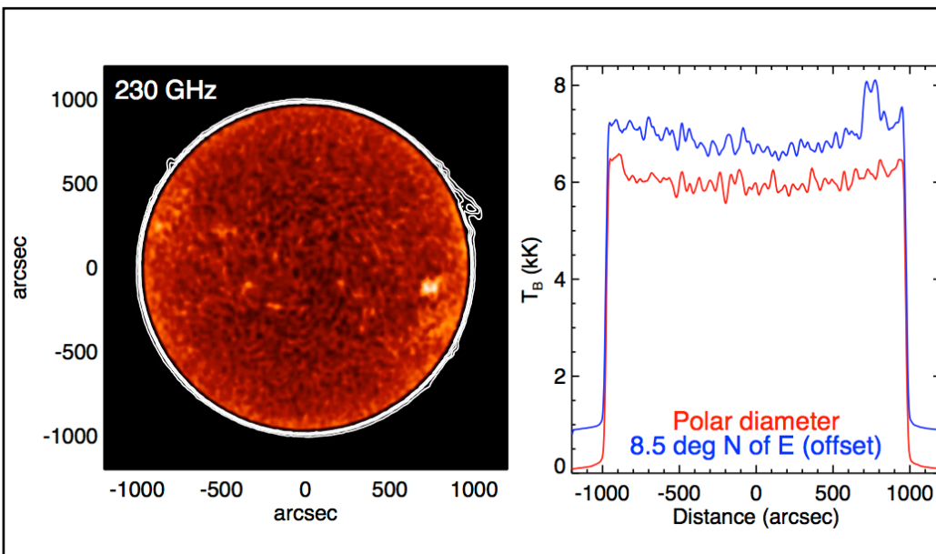
Figure 26: The left panel shows a 230 GHz (band 6) image of the Sun on 7 December 2016. In order to emphasize structure on the disk, the 230 GHz image color display ranges from 5300 to 7400 K. Low-level contours are plotted at 300, 600, 1200, and 2400 K in order to show features above the limb. The right panel shows disk profiles through the Poles and on a diameter through the active region in the southwest quadrant, but with the blue curve offset by 800 K in order to show structure in both. (Credit: ALMA (ESO/NAOJ/NRAO); S. White et al., 2017, SoPh , 292, 88)
