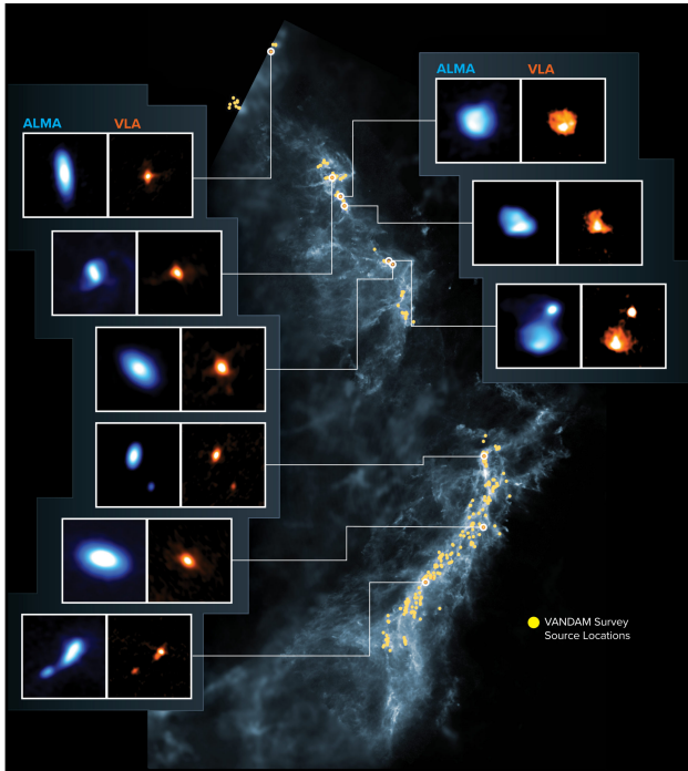
Figure 19: The VLA/ALMA Nascent Disk and Multiplicity (VANDAM) survey imaged more than 300 protoplanetary disks in the Orion molecular cloud (OMC). This image shows the OMC in blue (from Herschel), the observed protostars in the survey (yellow dots), and inset are a few of the disks imaged by ALMA (blue) and the Jansky VLA (orange). (Credits: ALMA (ESO/NAOJ/NRAO), J. Tobin; NRAO/AUI/NSF, S. Dagnello; Herschel/ESA; Tobin et al., 2020, ApJ , 890, 130)
