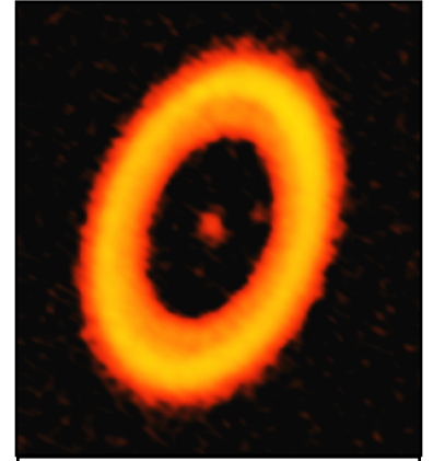
Figure 18: ALMA Band 7 image of the dust in PDS 70, a star system located approximately 370 light-years from Earth. Two faint smudges in the gap region of this disk are associated with newly formed planets. One such concentration of dust is a circumplanetary disk, the first such feature ever detected around a distant star. (Credits: ALMA (ESO/NAOJ/NRAO); A. Isella et al., 2019, ApJ , 879, L25)
