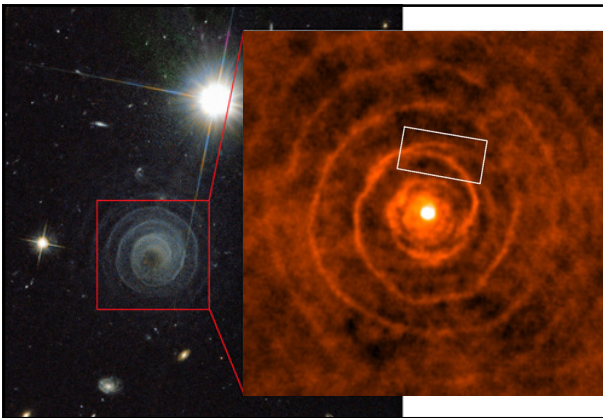
Figure 23: (left) HST image and (right) ALMA image of an expanding spherical shell and spiral wind emanating from the evolved star R Sculptoris. Recent modelling suggests that the bifurcation of the spiral-shell pattern (indicated by a white box) results from a highly elliptical binary system. (Credit: ESA/NASA & R. Sahai. (Right) ALMA image of LL Pegasi. Credit: ALMA (ESO/NAOJ/NRAO) / Kim et al., 2016, NatAs, 1, 60)
