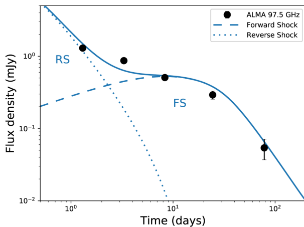
Figure 16: GRB161219B was observed by ALMA at Band 3 over five epochs ranging from 1.3 days to 78 days after the burst. On the left above, the Band 3 flux density is plotted as a function of time. The rebound, or reverse shock, triggered by the GRB's powerful jets slamming into surrounding debris, lasted thousands of times longer than expected. On the right is an artist's impression of the “reverse shock” echoing back through the jets of the GRB. (Credits: Laskar et al., 2018, ApJ, 862, 94L; NRAO/AUI/NSF, S. Dagnello)
