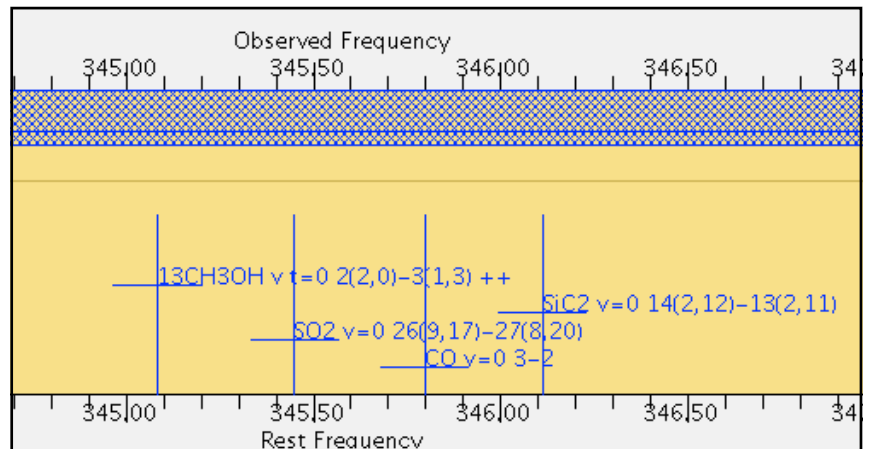
Figure 36: Four spectral windows were set up to observe these four lines simultaneously in one baseband using the OT. The windows are each 234 MHz wide (with 0.43 km/s channels), and are centered at 345.80, 345.45, 346.11 and 345.09 GHz. The spectral windows must fit within the 2 GHz wide baseband.
