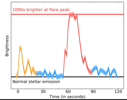
Figure 37: New analysis of ALMA observations reveal that Proxima Centauri emitted a powerful flare that would have created inhospitable conditions for planets in that system. Here is shown the brightness of Proxima Centauri as observed by ALMA over the two minutes of the event on March 24, 2017. The massive stellar flare is shown in red, with the smaller earlier flare in orange, and the enhanced emission surrounding the flare that could mimic a disk in blue. At its peak, the flare increased Proxima Centauri's brightness by 1,000 times. (Credit: M. MacGregor et al., 2018, ApJL , 855, 2)
