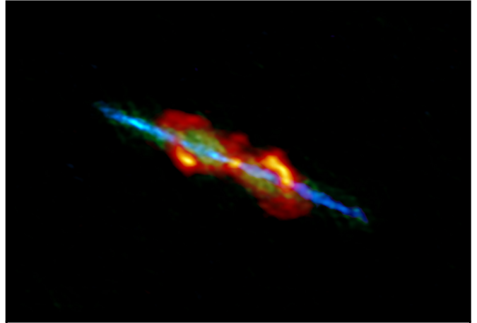
Figure 22: The asymptotic giant branch star W43A was observed by ALMA at Band 6, to understand how bipolar proto-planetary nebulae are generated. Here CO(J=2-1) emission clearly shows a high velocity jet (blue) ejected from the aged central star, within a lower velocity (green), with the dusty envelope of the star entrained by the jets shown in orange. (Credits: ALMA (ESO/NAOJ/NRAO); Tafuya et al., 2020, ApJ, 890, L14)
