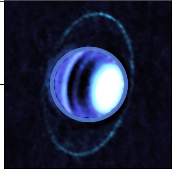
Figure 27: Composite image of Uranus's atmosphere and rings obtained using ALMA in December 2017. The image shows thermal emission from the rings of Uranus for the first time, enabling scientists to determine their temperature is a frigid 77 K. Dark bands in Uranus's atmosphere at these wavelengths are due to different optical depths of the bands, with the brightest regions (e.g. north polar region) indicating the greatest depth and highest temperature. (Credits: ALMA (ESO/NAOJ/NRAO); E. Molter and I. de Pater; Molter et al., 2019, AJ, 158, 47)
