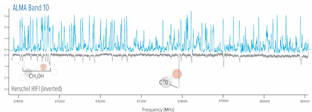
Figure 30: The upper blue portion of this graph shows the spectral lines ALMA detected in the NGC6334I star-forming region. The lower black portion shows the lines detected by the European Space Agency's Herschel Space Observatory. The ALMA observations detected more than ten times as many spectral lines. Note that the Herschel data have been inverted for comparison. Two molecular lines are labeled for reference. (Credit: NRAO/AUI/NSF, B. McGuire et al., 2018, ApJ, 863, L35)
