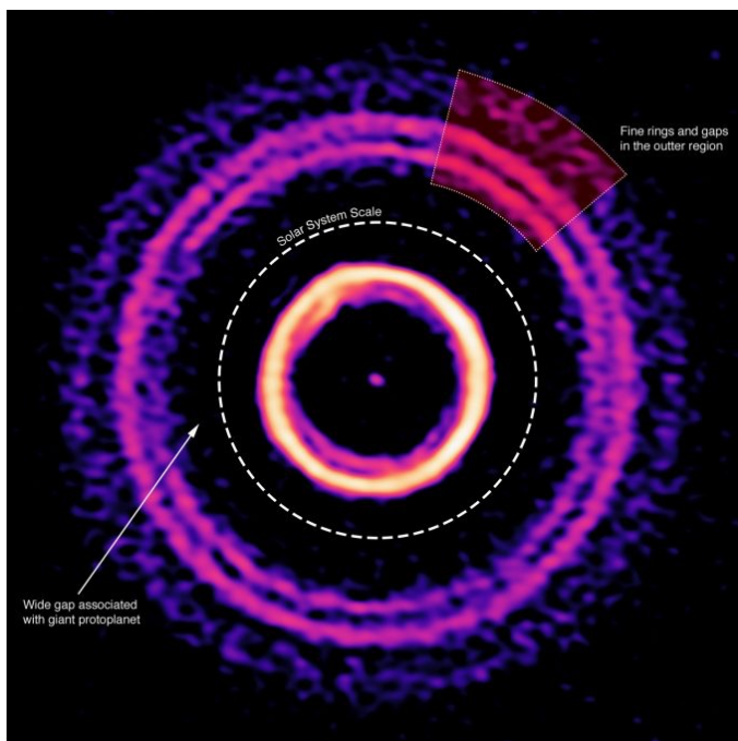
Figure 35: ALMA observations of the protoplanetary disk around HD169142 which shows an outer region composed of thin rings and a double gap. The image also reveals a bright inner ring with signs of being subject to dynamical perturbations, possibly by a “mini-Neptune”-size planet. Solar system size approximated by Pluto’s orbit is shown for comparison. (Credits: N. Lira – ALMA (ESO/NAOJ/NRAO); S. Pérez – USACH/UCHile.)
