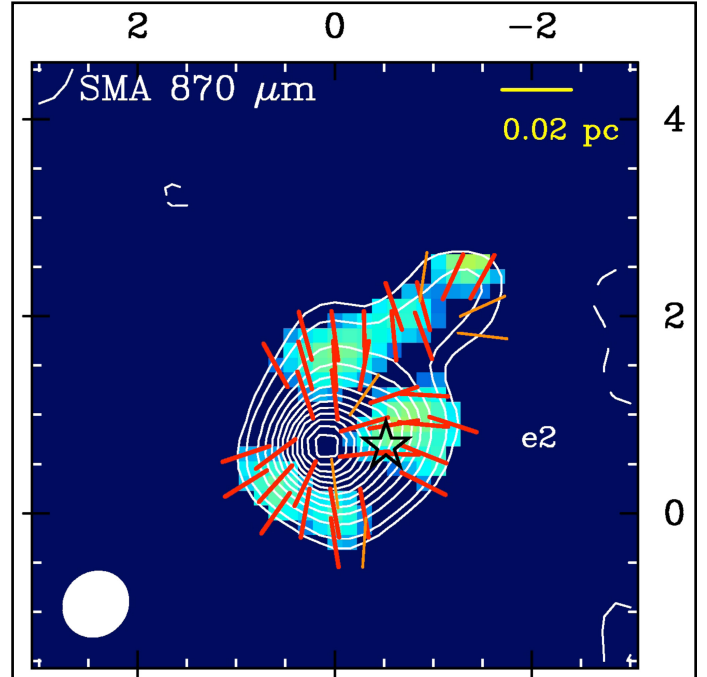
Figure 20: Magnetic field of the W51 e2 core at 0.9 mm obtained at the Submillimeter Array. The total intensity is shown in contours. The polarization intensity is shown in color scale. The star denotes the ultracompact HII region. (Credit: Ya-Wen Tang, 2009 ApJ, 700, 251)
