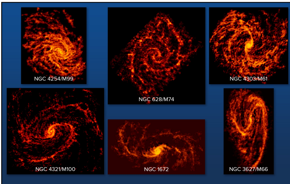
Figure 17: Six of the galaxies imaged using mosaics of 12-m, 7-m, and TP Arrays in the 2017 Large project to image 100,000 giant molecular clouds in 74 nearby galaxies. These results have been presented in a series of papers in the Astrophysical Journal and Astrophysical Journal Letters . (Credit: ALMA (ESO/NAOJ/NRAO); NRAO/AUI/NSF, B. Saxton; J. Sun et al., 2018, ApJ , 860, 172)
