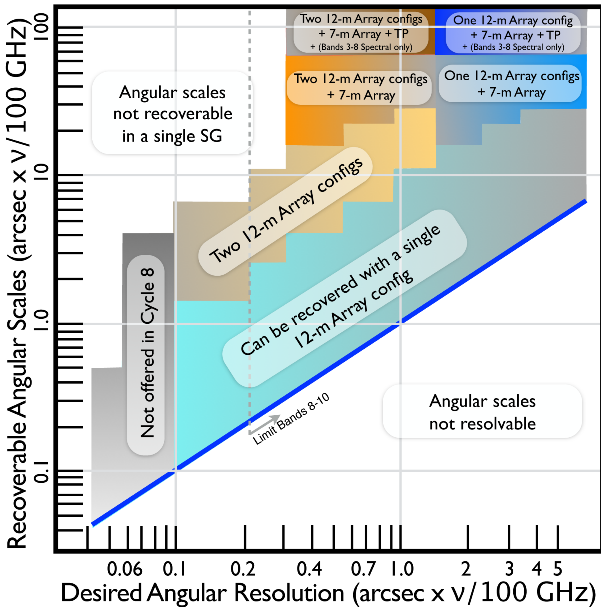
Figure 28: This figure links Desired Angular Resolution to the Maximum Recoverable Scale (MRS). The desired angular resolution determines the largest baselines (and hence the configuration) of the 12-m Array. The observations from that configuration can recover structure over a range of angular scales; for example, an observation at 1" resolution at 100 GHz can recover structure over size-scales from ~1" to ~11" (cyan region). Structures larger than the "Maximum Recoverable Scale" (MRS; see p. 24) are "resolved out" by the interferometer. Structure larger than the MRS may be recovered either by adding observations using a smaller 12-m Array configuration, by adding observations using the 7-m Array, or by adding both another configuration and the 7-m Array. Still larger scale structure may be recovered for Bands 3-8 spectral observations by adding data from the Total Power (TP) array. To use this figure, you first need to scale your desired angular resolution and LAS by the factor (\nu/100\text{GHz}) , where \nu is your desired frequency in GHz. For example, suppose you wanted to observe at 300 GHz (Band 7) with angular resolution 0.4" and LAS of 10". These become 1.2" and 30" respectively when scaled to 100 GHz. Reading from the figure above, two 12-m Array configurations plus the ACA 7-m Array would be needed to recover all angular scales. (The OT will automatically determine the required combination of arrays/configurations to achieve the resolution/LAS you require.) Note that adding configurations or the ACA will significantly increase the required observing time. See Chapter 7 of the Technical Handbook and the Proposer's Guide in the Call for Proposals for details and restrictions. Note that angular resolutions finer than (0.21" \times 100\text{GHz}/\nu) are not permitted for Bands 8-10 (Limit Bands 8-10 on figure above). The two largest configurations (C-9, C-10) are not offered in Cycle 8.
