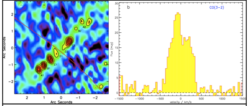
Figure 12: (a) SMA (very extended configuration) 870 \mu\text{m} image of the Cosmic Eyelash. The red line marks the division between the two images of the background source. (b) Spectrum of CO(3-2) taken with the Plateau de Bure interferometer. Both figures are from Swinbank et al. (2010, Nature , 464, 733).
