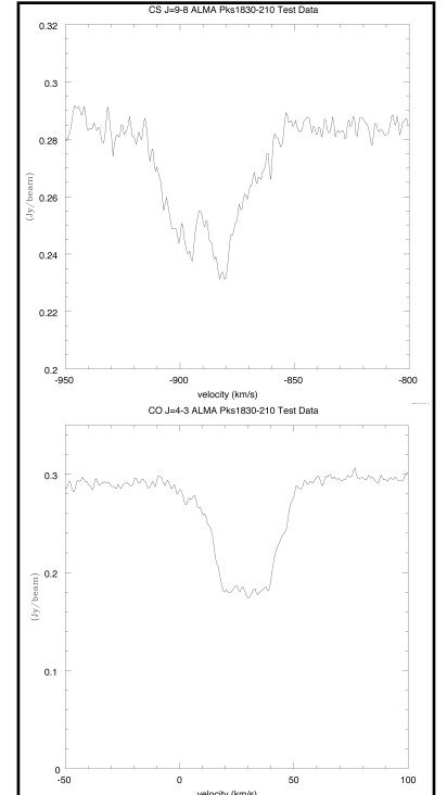
Figure 11: Examples of molecular absorption lines detected toward PKS1830-211. These observations were made by ALMA in late 2010 when there were only a few antennas.
