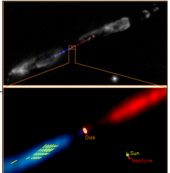
Figure 21: ALMA was used to detect the magnetic field in the jet from a protostar, using polarized SiO line emission. The top image (right) shows an optical H 2 image of the HH 211 jet (from Hirano et al. 2006). The blue and red features show the blue- and red-shifted SiO J=8-7 emission. The inset image shows the inner jet, with the recently detected disk (Lee et al. 2018), the solar system scale for comparison, and yellow bars showing the SiO line polarization vectors. The vector orientations are consistent with a model of a helical magnetic field threading the jet. (Credit: ALMA (ESO/NAOJ/NRAO); Lee et al., 2018, NatCo, 9.4636)
