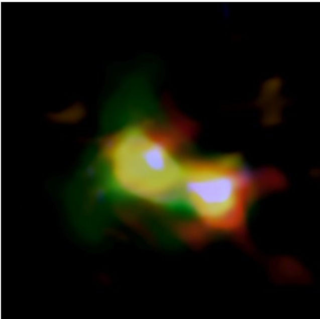
Figure 15: ALMA observed the earliest known example of a merging (non gravitationally lensed) galaxy. This image of B14-65666, a Lyman break galaxy at z=7.15 , shows the distribution of dust (in red), oxygen (in green), and carbon (in blue), observed by ALMA, plus stars (in white) from the HST. (Credits: ALMA (ESO/NAOJ/NRAO), NASA/ESA Hubble Space Telescope, Hashimoto et al., 2019, PASJ , 71, 71)
