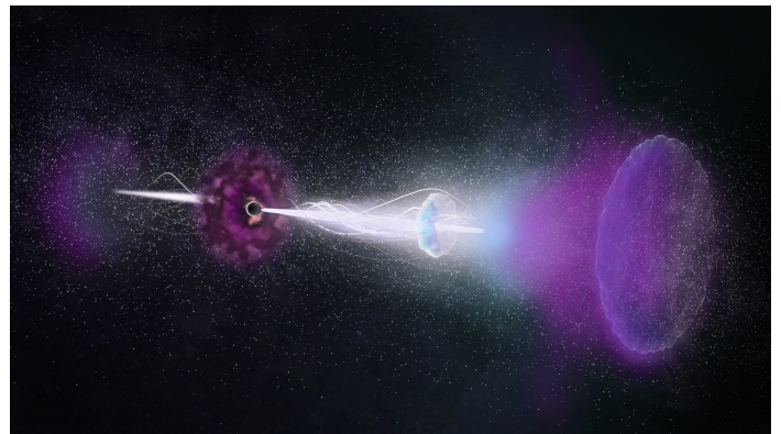
Figure 16: GRB161219B was observed by ALMA at Band 3 over five epochs ranging from 1.3 days to 78 days after the burst. On the left above, the Band 3 flux density is plotted as a function of time. The rebound, or reverse shock, triggered by the GRB's powerful jets slamming into surrounding debris, lasted thousands of times longer than expected. On the right is an artist's impression of the “reverse shock” echoing back through the jets of the GRB. (Credits: Laskar et al., 2018, ApJ, 862, 94L; NRAO/AUI/NSF, S. Dagnello)
