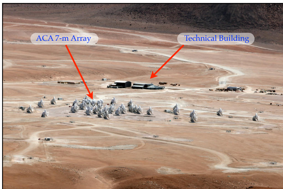
Figure 6: An areal view of ALMA in a relatively compact configuration. The maximum distance between the 12-m Array antennas in the most compact configuration is about 150 m, and the minimum distance a mere 15 m. Indicated also are the AOS Technical Building, and the ACA 7-m Array. (Credit: C. Padilla/ALMA (ESO/NAOJ/NRAO))
