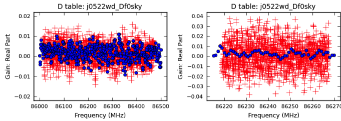
Figure 8.5: A close-up view in frequency space of the real part of D -term shown in Figure 8.4. Blue circles and red crosses are showing the D -terms obtained from setup #1 (FDM, 2 GHz bandwidth) and setup #2 (FDM, 500 and 62.5 MHz bandwidth respectively).
