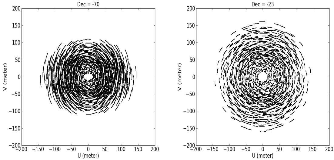
Figure 7.8: uv plane coverage for notional configuration C43-1 with a 1-hour observation of a transiting source at a declination of either -70^\circ ( left ) or -23^\circ ( right ). For the source with a declination of -70^\circ , 25.7% of visibilities are expected to be flagged due to shadowing.
