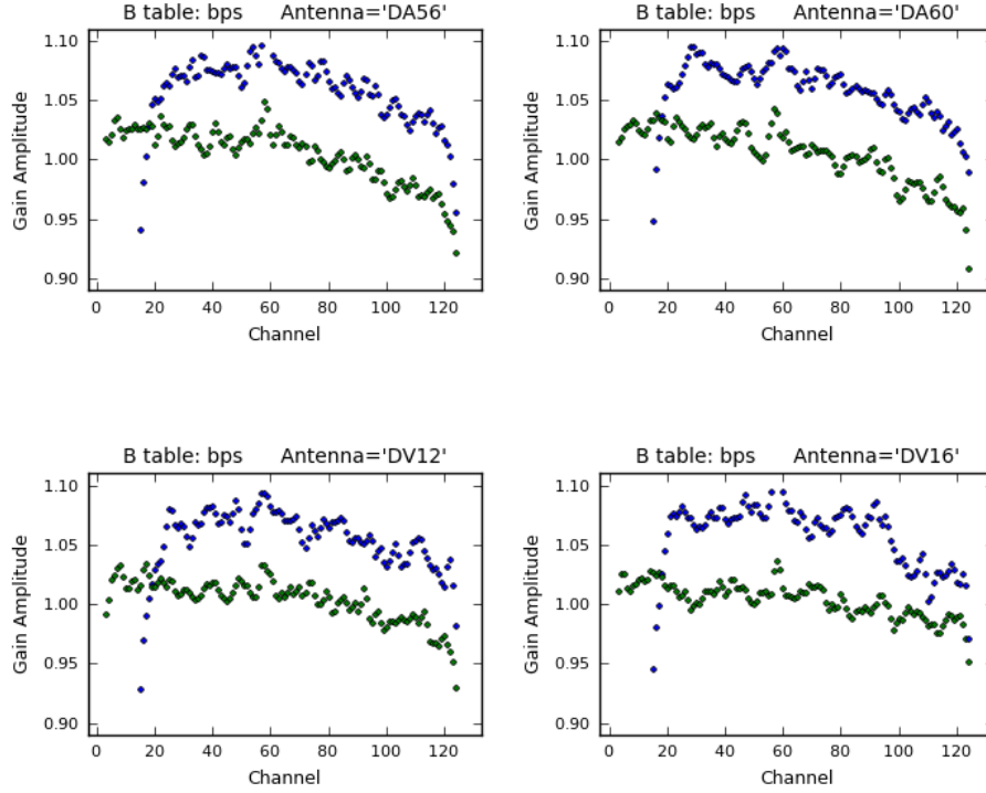
Figure 10.5: Bandpass Amplitude: The bandpass amplitude at Band 9 for four antennas, Xpol are shown as blue dots and Ypol as green dots. Xpol channels below 10 and Ypol channels above 120 should be flagged. Notice that the line emission near channel 60, seen in the T_{sys} solution (Figure 10.2), has been significantly reduced after multiplication of the raw visibility amplitude by the T_{sys} factor.
