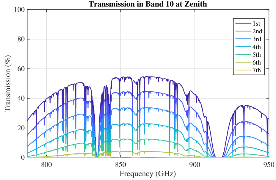
Figure 4.34: Band 10 zenith transmission for the first seven octiles of observing conditions at ALMA. Transmission of most of the band is affected by the wings of pressure-broadened lines of \text{H}_2\text{O} at 841 and 916 GHz.
