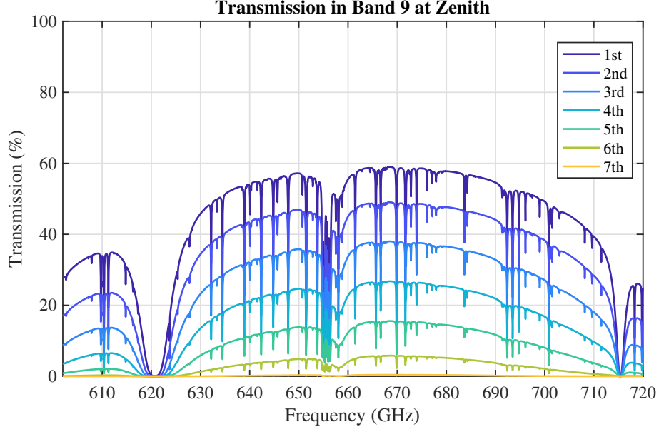
Figure 4.30: Band 9 zenith transmission for the first seven octiles of observing conditions at ALMA. Most of the band is affected by the wings of pressure-broadened \text{H}_2\text{O} at 620 GHz.
