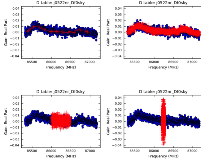
Figure 8.4: A frequency vs real part of the D-terms plot for an antenna (DV22) obtained towards J0522-364. Blue circles and red crosses are showing the D-term obtained using a setup of FDM with 2 GHz bandwidth and using a setup with higher spectral resolutions (FDM 500 and 62.5 MHz bandwidth respectively). Four panels show the D-terms obtained from the spw 0, 1, 3, 2 (from top left, clockwise).
