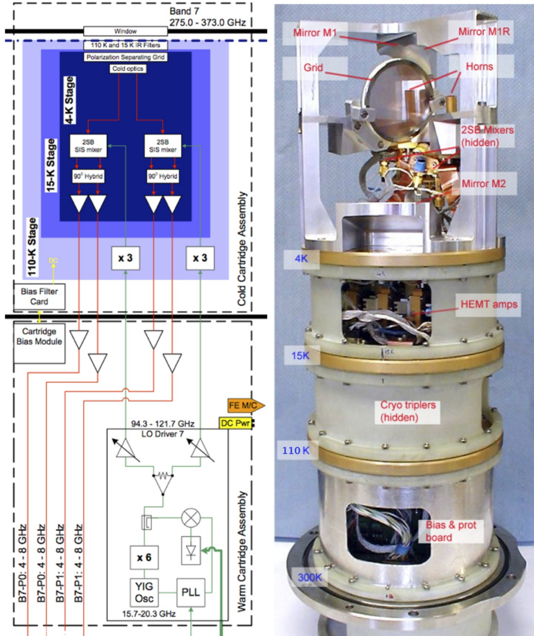
Figure 4.21: Band 7 front-end receiver block diagram, and (right) annotated image of the Band 7 cartridge. Note the polarization-splitting grid and LO injection in the cold optics above the mixers. The Band 7 cartridges were built in France at the Institut de Radio Astronomie Millimétrique (IRAM) in Grenoble, France.
