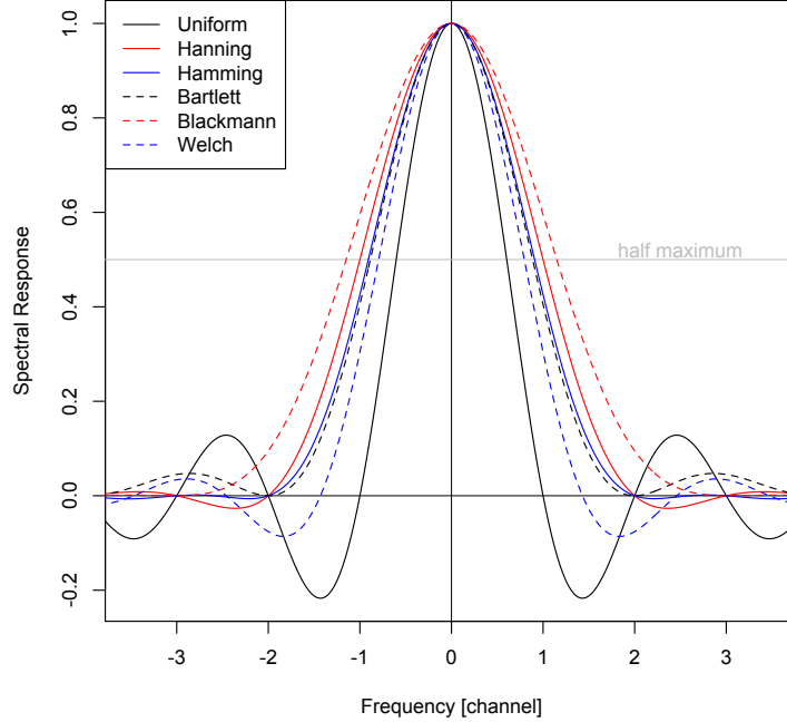
Figure 5.7: (left table) Spectral resolutions (FWHM) and the maximum sidelobe levels for weighting functions. ALMA employs the Hanning window in default. (right figure) Spectral resolution functions corresponding to various weighting functions
