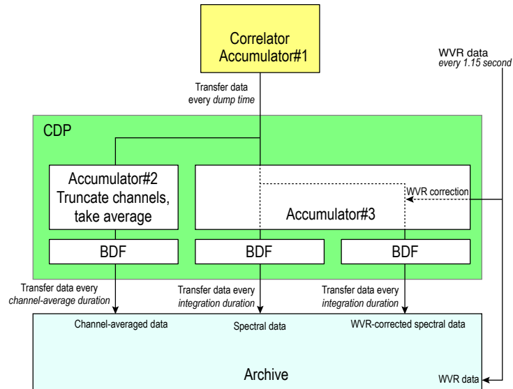
Figure 5.8: Basic data processing and accumulation/averaging steps between the correlator and archive. The CDP applies channel truncation, spectral averaging, and time averaging for the channel-averaged data. It also applies online WVR correction to produce the WVR-corrected spectral data. They are packed in Binary Data Format (BDF) and are archived together with the WVR data.
