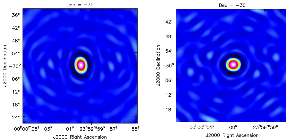
Figure 7.7: Beam shape for notional configuration C43-1 with a 2-hour observation of a transiting source at a declination of either -70^\circ (left) or -30^\circ (right).
