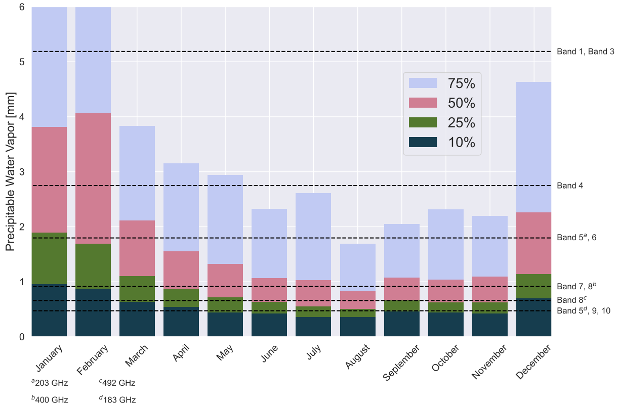
Figure 2: Fraction of time that the PWV falls below a given value along the year. The percentages shown indicate the fraction of time that the PWV is under the PWV value indicated on the y-axis. For example, in March 75% of the PWV measurements are under 3.8 mm, and in June 75% of the PWV measurements fall below 2.3 mm. The data were obtained with the APEX weather station, ALMA measurements, and weather forecast data between January 2010 and January 2022. The horizontal dashed lines show the PWV observing limits adopted for the ALMA bands for an elevation of 60 degrees.
