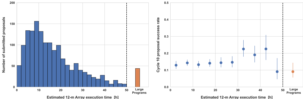
Figure 1: (Left) Number of proposals submitted as a function of the 12-m Array execution time in Cycle 10. (Right) The fraction of proposals (with 1\sigma confidence intervals) that were assigned priority Grade A or B as a function of the estimated 12-m Array time.
